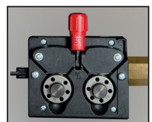
Trainafilo 4 rulli D.37mm 4 rolls wire feeder D.37mm
